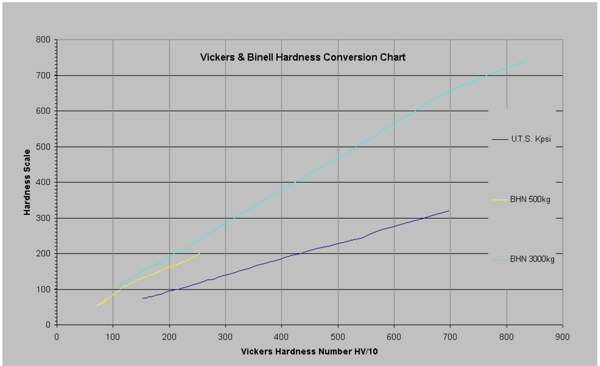
Brinell and Vickers Hardness Scale and Tensile Strength Comparison Chart
