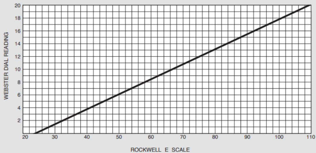
HARDNESS CONVERSION FOR ALUMINUM ALLOYS MODEL B
