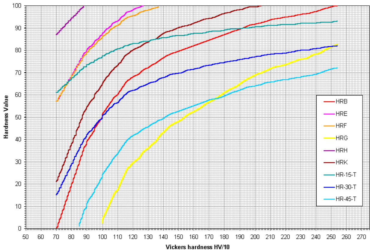
Hardness Conversion Chart for Soft Metals (Rockwell B Scale)
