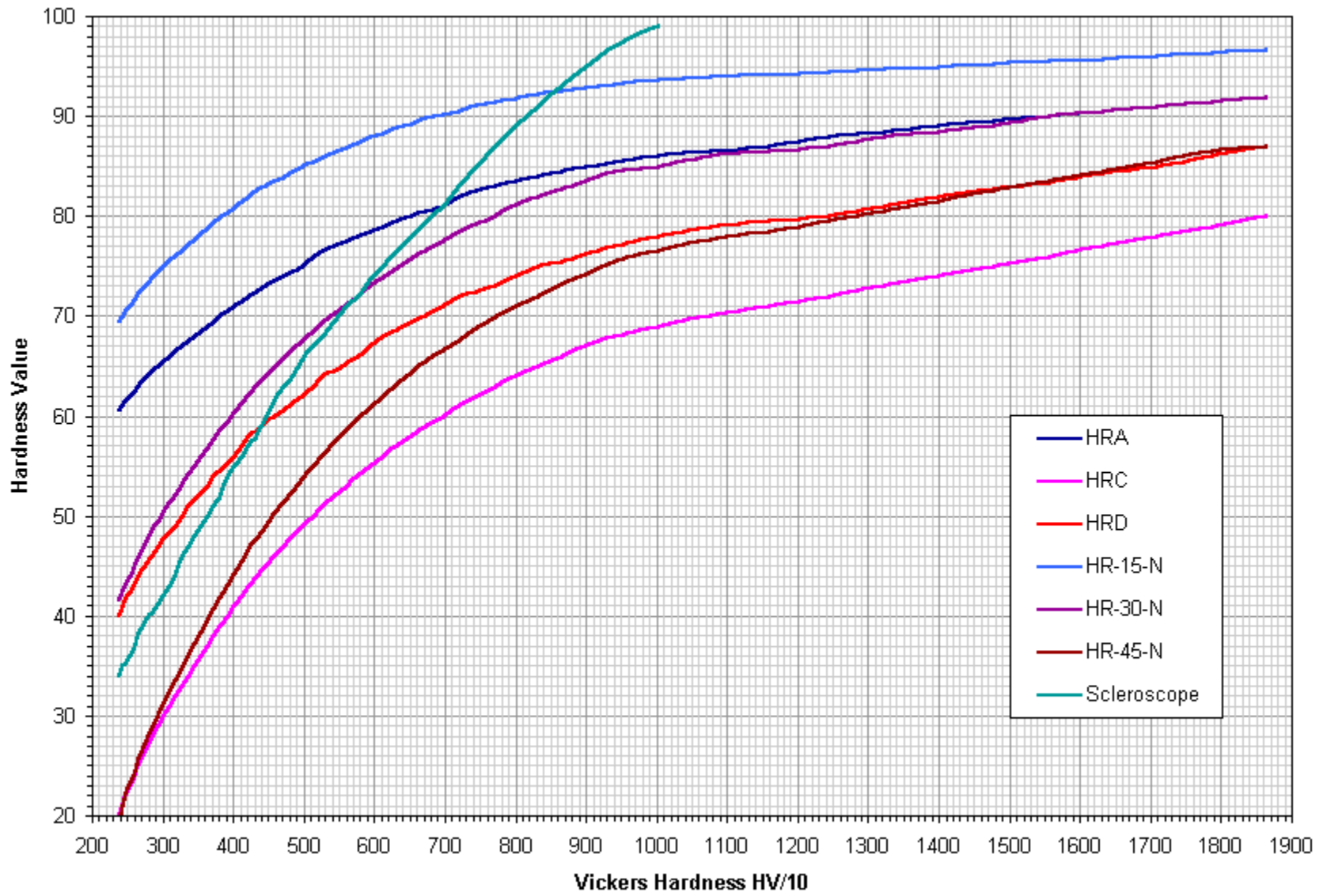
Hardness Equivalence Chart for Hard Materials (Rockwell C range)
